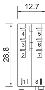
BOTTOM VIEW
